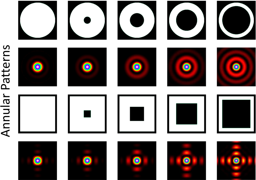
Diffraction Patterns
